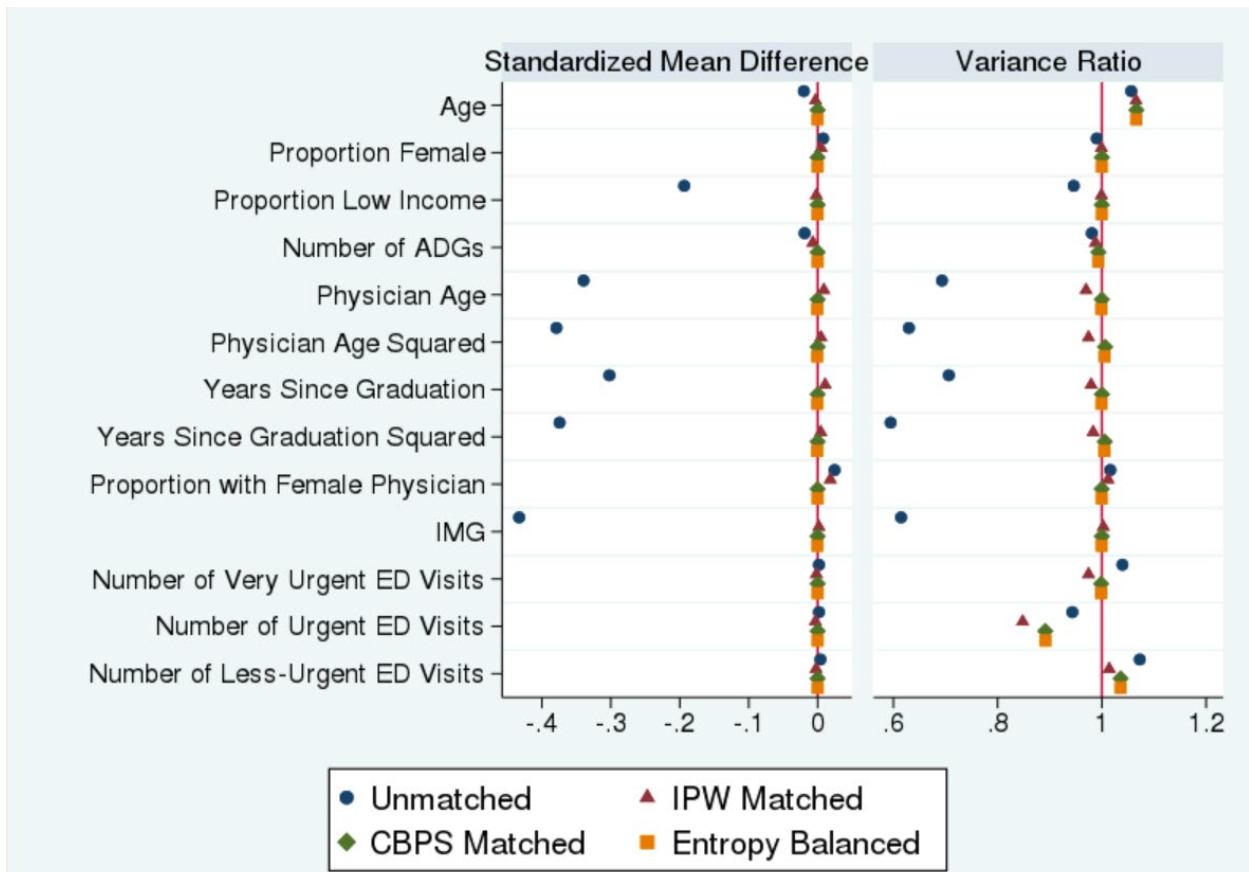
Figure A2. Standardized mean difference and variance ratio before and after weighting using propensity score weighting and entropy balancing
