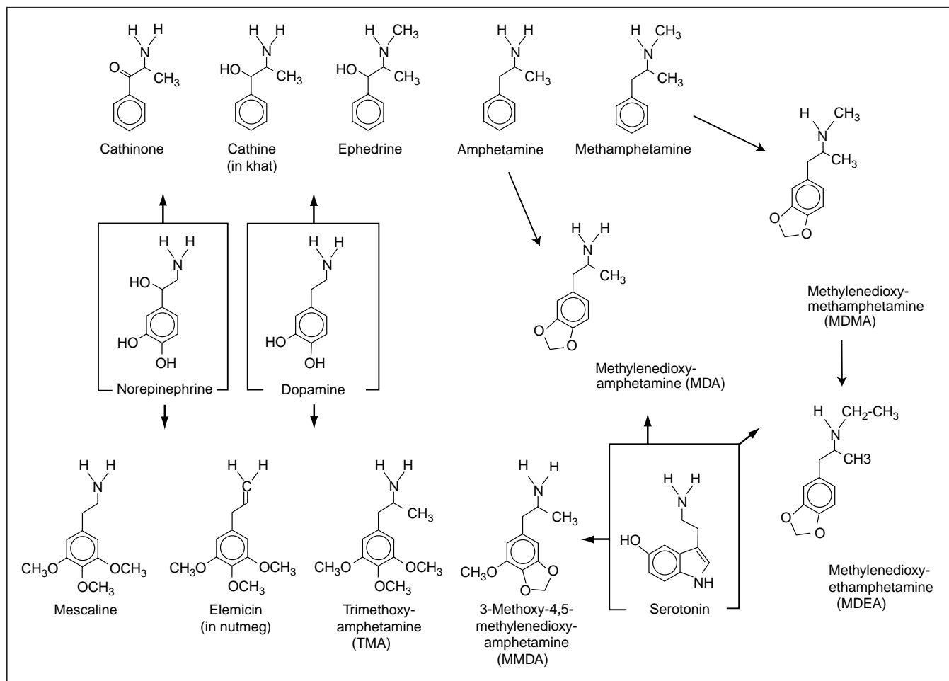
Fig. 1: Chemical structures of MDMA, MDEA and related drugs compared with those of the monoamine neurotransmitters. Arrows do not represent pathways of synthesis or metabolism; they merely indicate the closest resemblances of structure.
